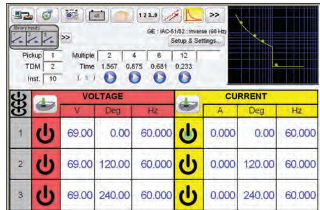
Figure 5. Timing Test Screen for G.E. IAC-51 Inverse Overcurrent Relay
